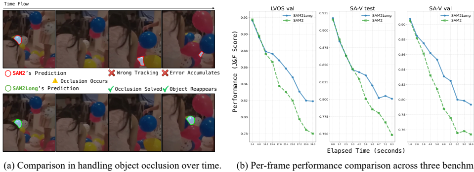
Figure 1: Comparison of occlusion handling and long-term capability between SAM 2 and SAM2Long. (a) When an occlusion occurs, SAM 2 may lose track or follow the wrong object, leading to accumulated errors. In contrast, SAM2Long utilizes memory tree search to recover when the object reappears. (b) The per-frame \mathcal{J}\&\mathcal{F} scores of the predicted masks are plotted at specific timestamps on the LVOS and SA-V datasets. SAM2Long demonstrates greater resilience to elapsed time compared to SAM 2, maintaining superior performance over longer periods.
