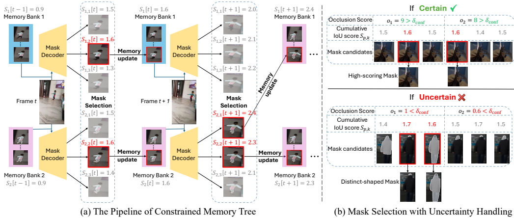
Figure 2: (a) The pipeline of constrained memory tree: At each time step t , we maintain multiple memory pathways, each containing a memory bank and a cumulative score S_p[t] . The input frame is processed through the mask decoder conditioned on the memory bank, generating three mask candidates for each pathway. The candidates with the highest updated cumulative scores S_{p,k}[t] are carried forward to the next time step. (b) Mask selection with uncertainty handling: When the maximum absolute occlusion score exceeds the threshold \delta_{\text{conf}} ( Certain ), the high-scoring mask is selected. Otherwise ( Uncertain ), distinct mask candidates are picked to avoid incorrect convergence.
