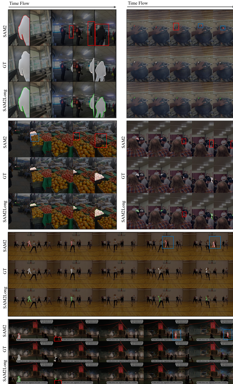
Figure 3: Qualitative comparison between SAM 2 and SAM2Long, with GT (Ground Truth) provided for reference. A blue box is used to highlight incorrectly segmented objects, while a red box indicates missing objects. Best viewed when zoomed in.
